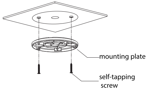
Figure 3-4 Installation step (1)
