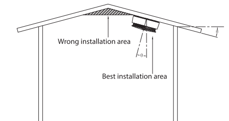
Figure 3-3 Installation position (2)
