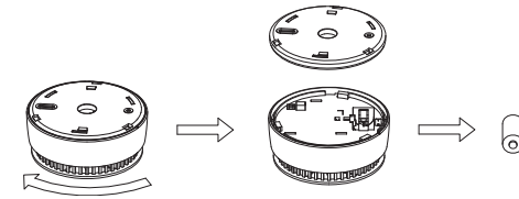
Figure 7-1 Battery replacement
