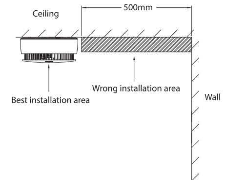
Figure 3-2 Installation position (1)
