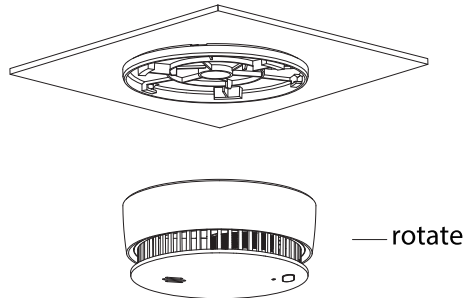
Figure 3-5 Installation step (2)
