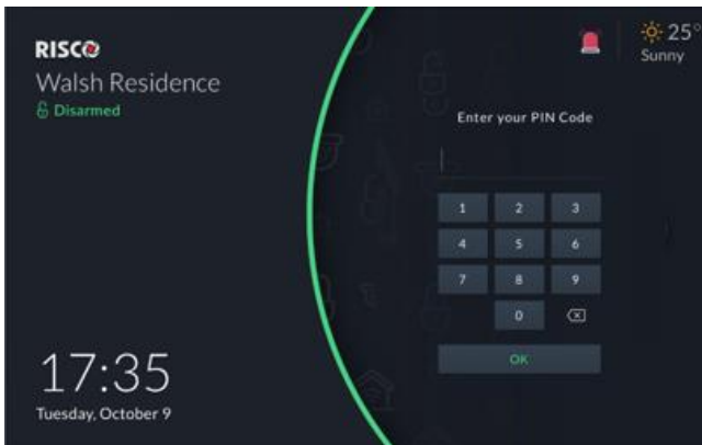
Figure 19: Lock Screens
